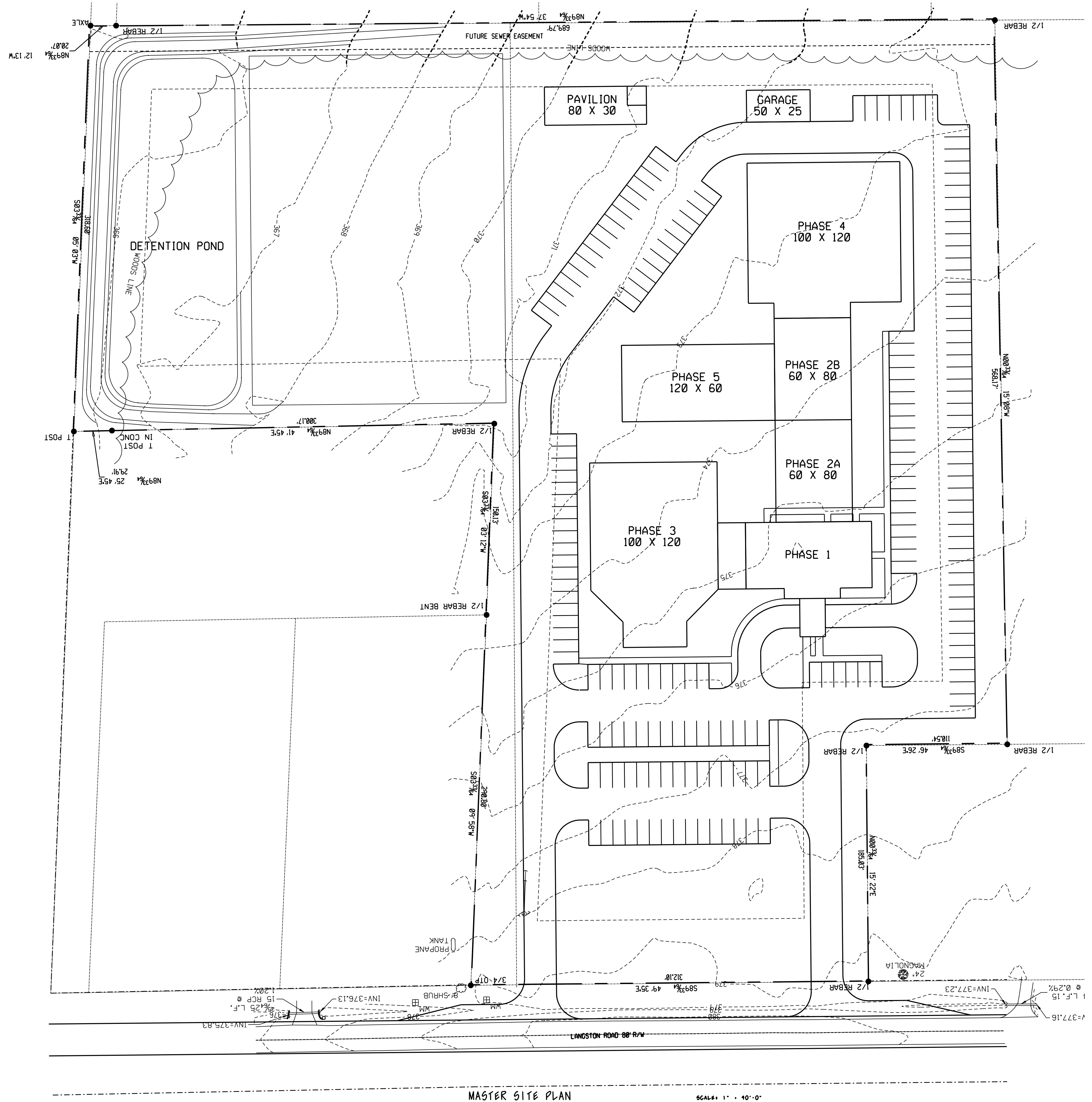
MASTER SITE PLAN
